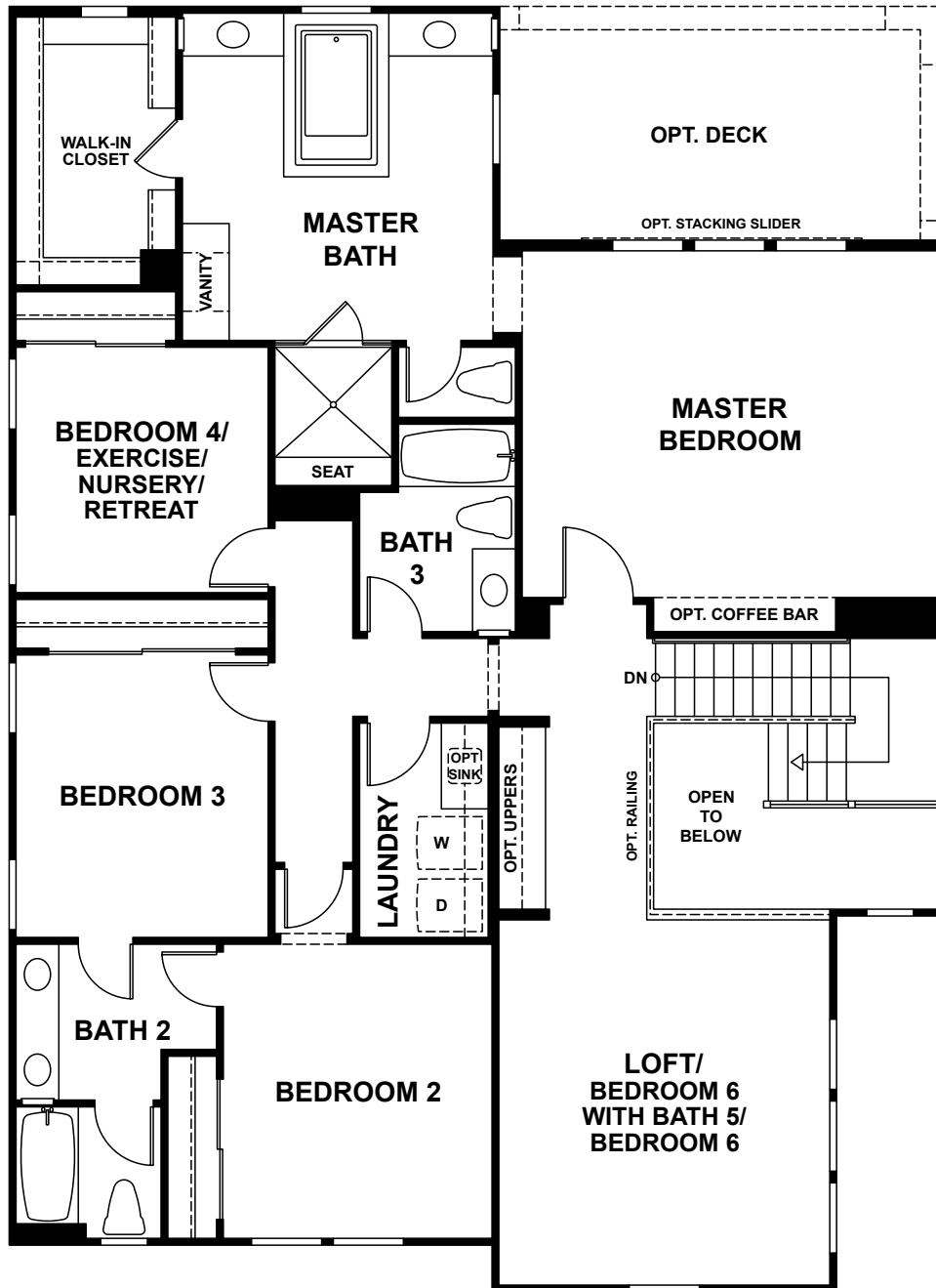
SECOND FLOOR
