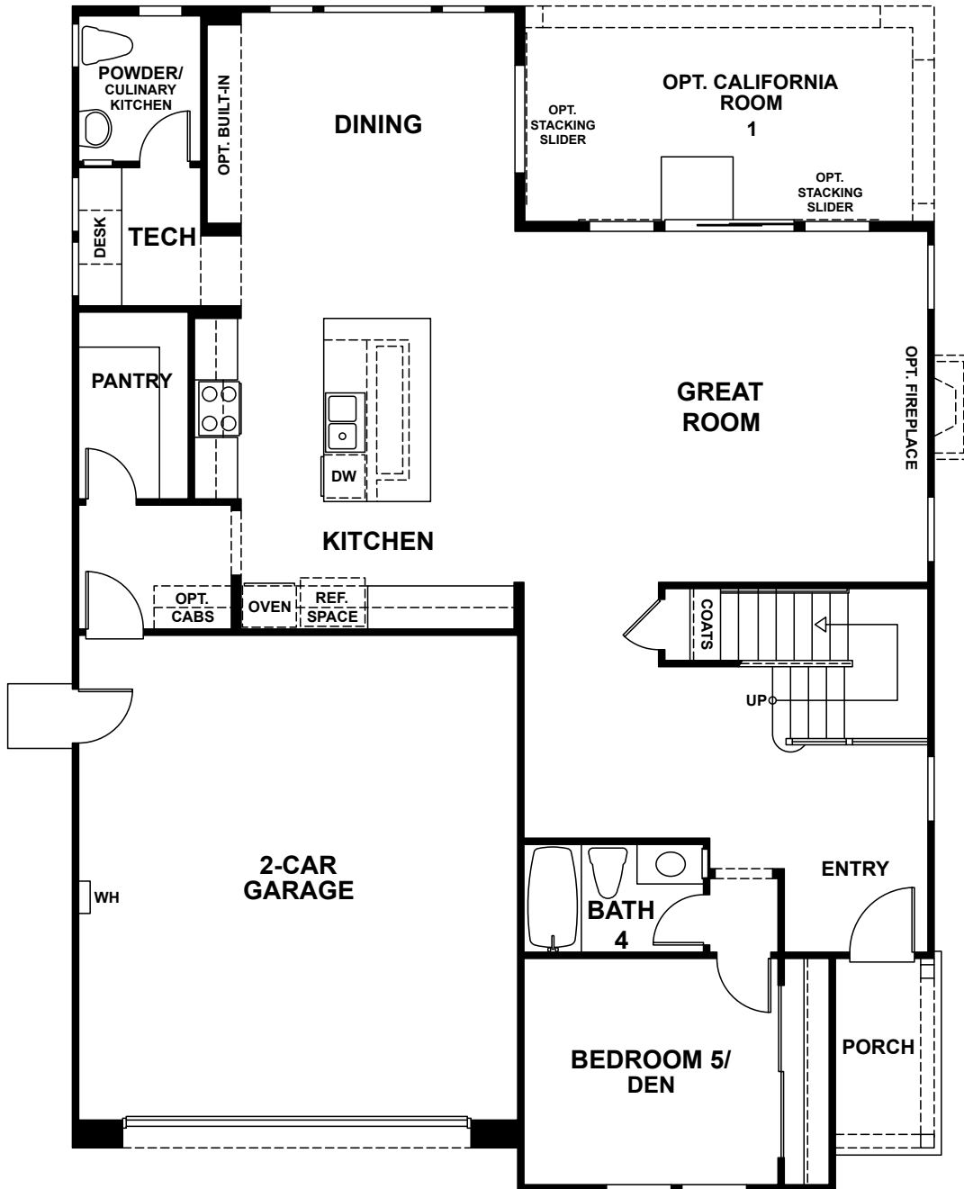
FIRST FLOOR
